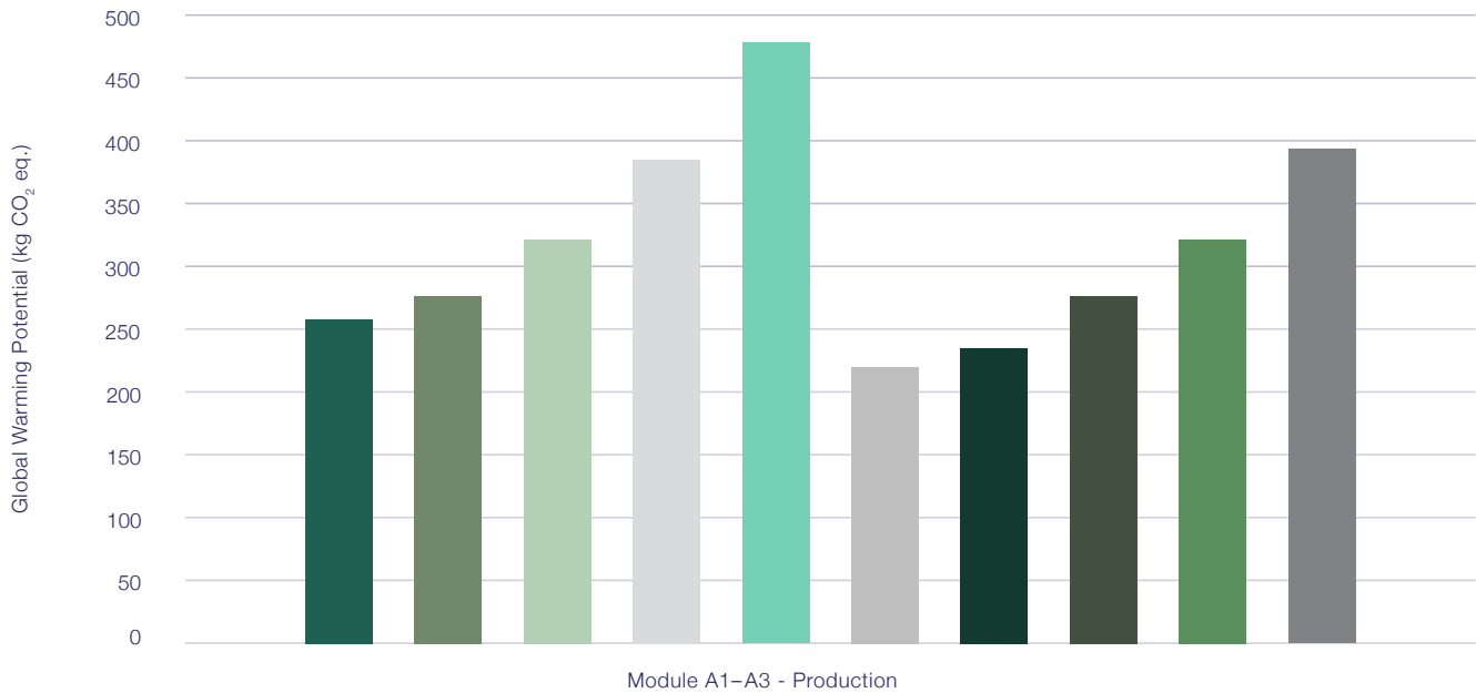
Figure 3 | Contributors to GWPT impacts of Adbri Normal Class Concrete in the different life cycle stages
