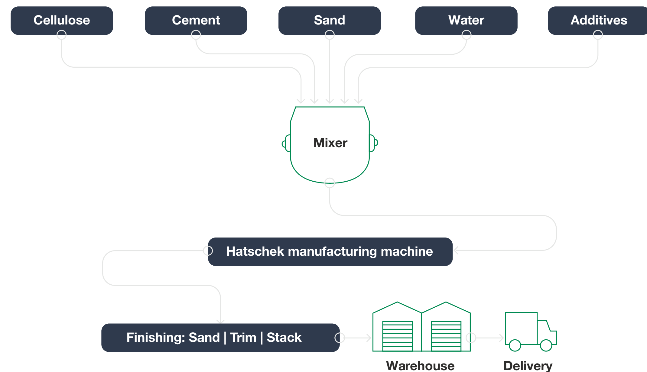
FIGURE 2 MANUFACTURING PROCESS
