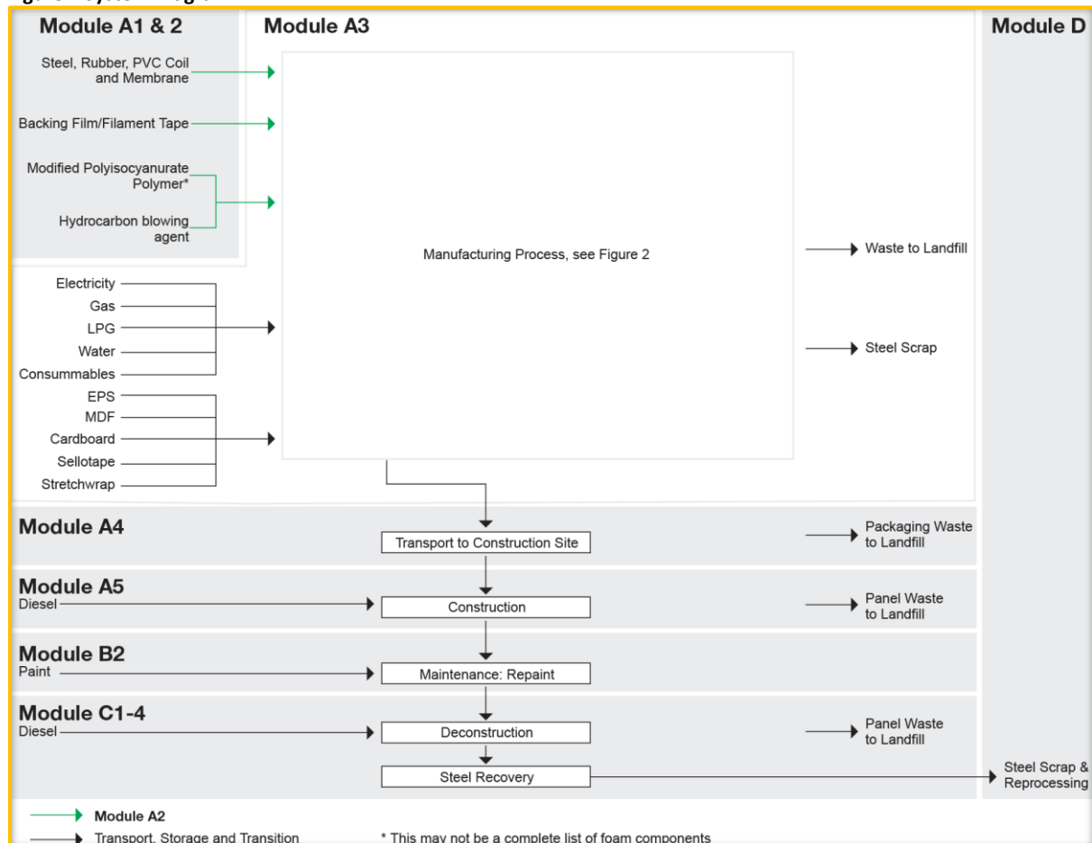
Figure 1 System Diagram
