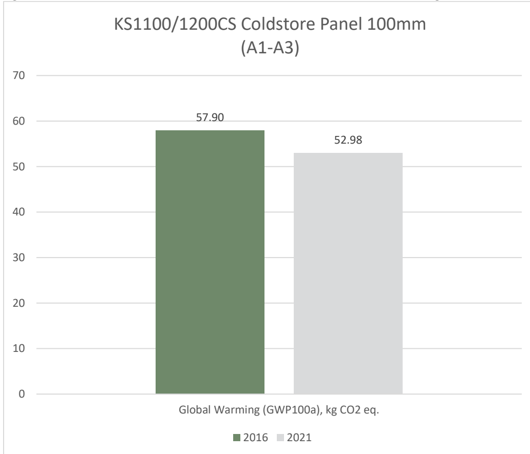
Figure 3: Benchmarked environmental results for KS1100/1200CS Coldstore Panels against 2016 results
